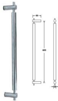
903.00.696 PULL BAR HANDLE SS MATT 600mm Packing: Set
