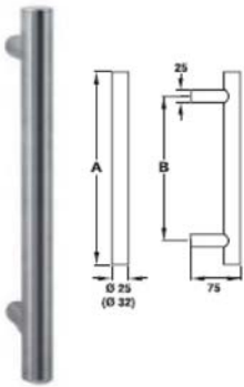
903.00.430 PULL BAR HANDLE D25mm, SS MATT 1,000mm
