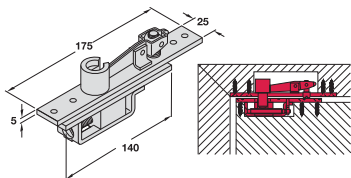
932.10.410 TOP PIVOT GEZE MIN HINGE WITHOUT ANGLE Packing: 1 pc
