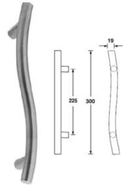
903.00.080 PULL BAR HANDLE SS MATT 300mm Packing: 1 Pair
