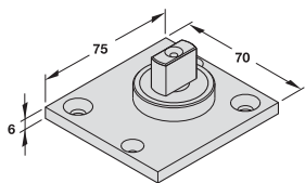
932.10.601 PIVOT BEARING GEZE, 250 Kg Packing: 1 pc
