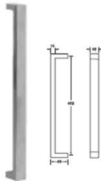
903.00.070 PULL BAR HANDLE SS MATT 450mm Packing: Set
