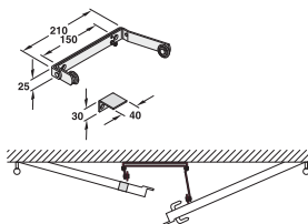
931.97.902 DOOR SELECTOR, CHR.PL. Packing: 1 set
