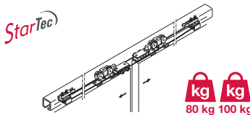
940.44.000 ADDITIONAL SET SILENT SYNCHRO, 60/A & 100/A
