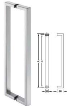
903.03.256 PULL BAR HANDLE SS MATT 630mm Packing: 1 Pair
