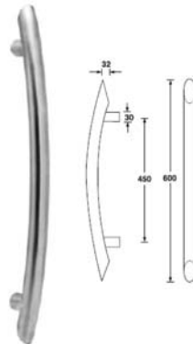
903.00.090 PULL BAR HANDLE SS MATT 600mm Packing: Set
