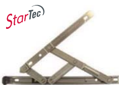
WINDOW FRICTION HINGE TOP HUNG 972.05.017 H1000mm/45 972.05.019 H1200mm/50 Packing: 1 Pair
