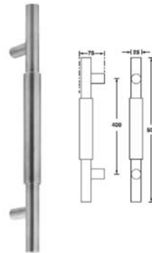
903.00.100 PULL BAR HANDLE SS MATT 500mm Packing: Set
