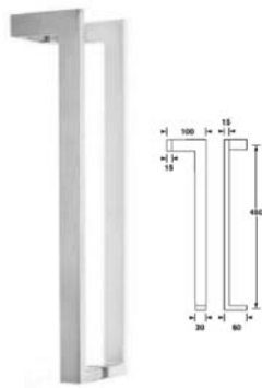
903.99.358 PULL BAR HANDLE SS MATT 450mm Packing: 1 Pair
