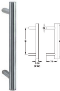
903.00.530 PULL BAR HANDLE D25mm, SS MATT 1,000mm
