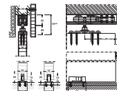
940.62.001 60/Slimline, FITTING SET FOR 1 DOOR. 1 set
